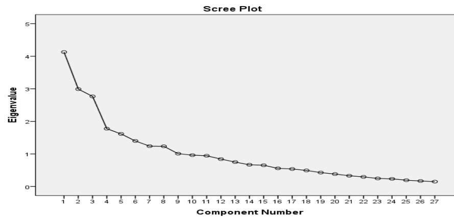
Figure 1: Scree plot
